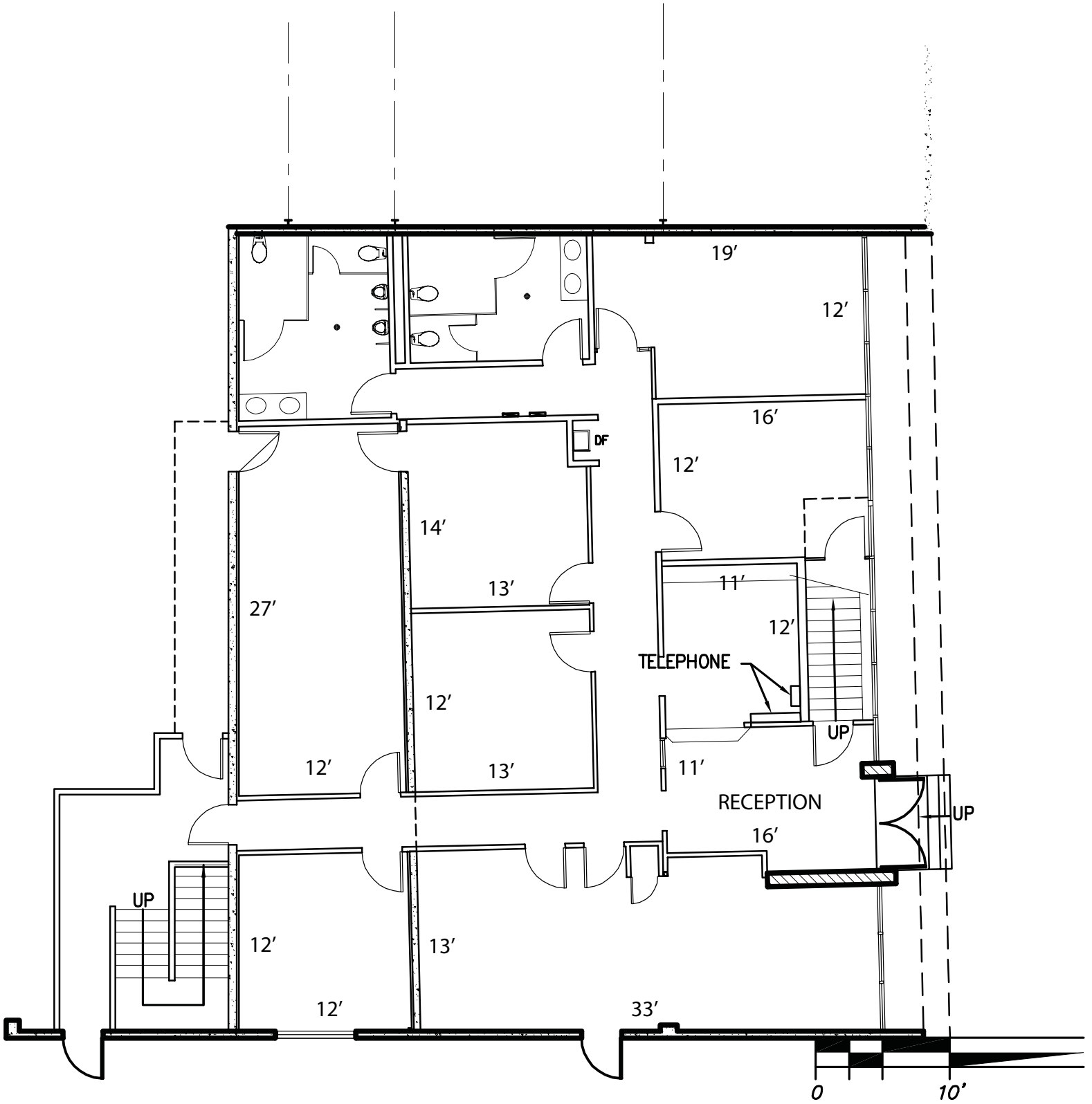
FIRST FLOOR
